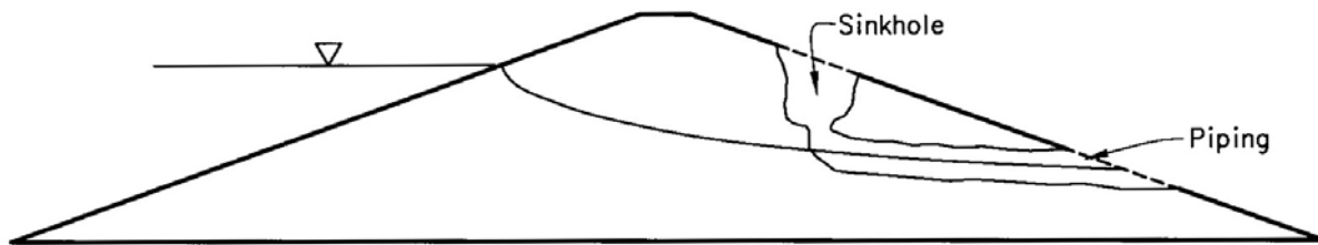
FIGURE II-12. FORMATION OF A SINKHOLE
