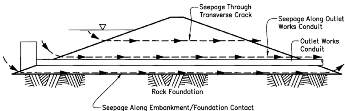
FIGURE II-6. Internal Erosion
