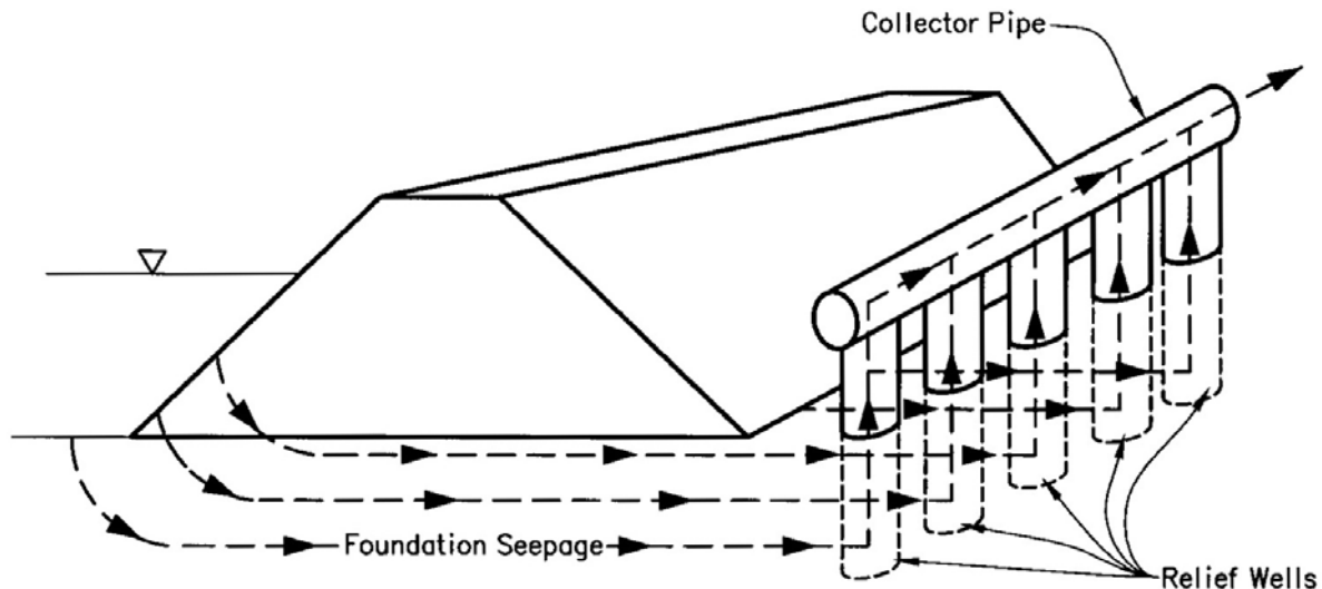
FIGURE II-3. RELIEF WELLS
